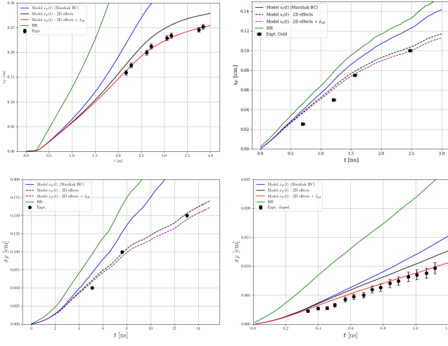
FIG. 2. Heat front position from the 1.5D model (solid curves) compared to experimental data (symbols) for four experiments: (a) Moore et al. [10], \text{C}_8\text{H}_7\text{Cl} ; (b) Back et al. [9], \text{Ta}_2\text{O}_5 ; (c) Back et al. [8], \text{SiO}_2 ; (d) Ji-Yan et al. [14], \text{C}_8\text{H}_8 .
